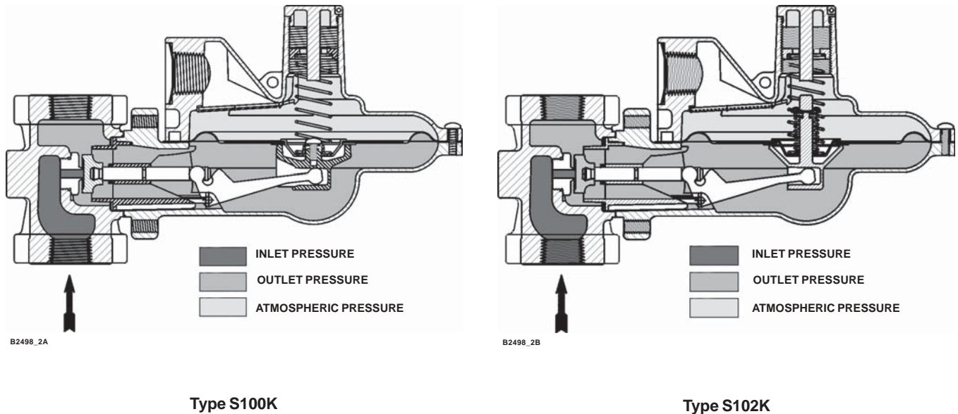
Figure 3. Types S100K and S102K Regulator Operational Schematics
