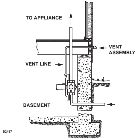
Figure 2. Typical Vent Line Installation
